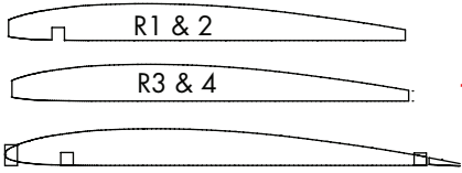
Wing Ribs R1 - 1 off 1.5mm balsa R2 - 2 off 0.8mm balsa R3 - 6 off 0.8mm balsa R4 - 2 off 1.5mm balsa
